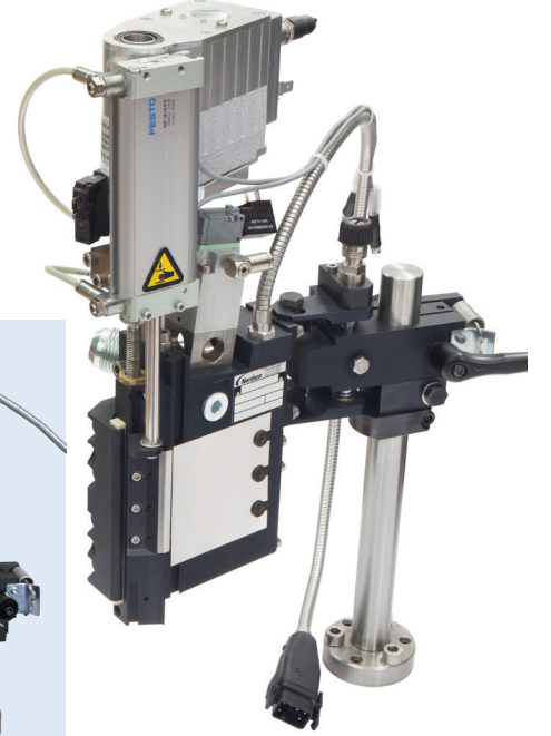
Motorized Adjust (Standard) Version
